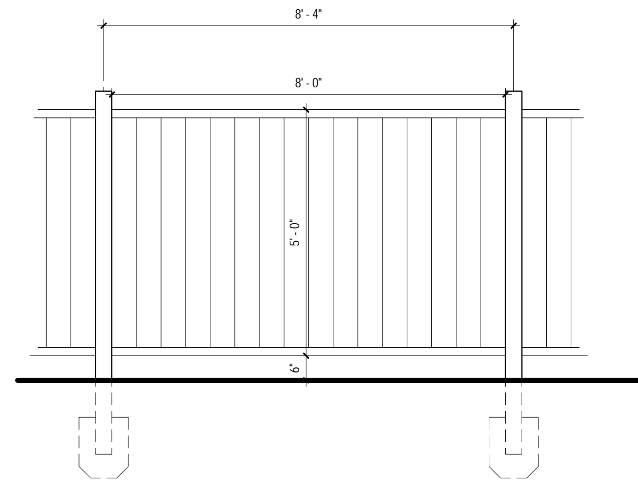
5' PANEL FENCE
