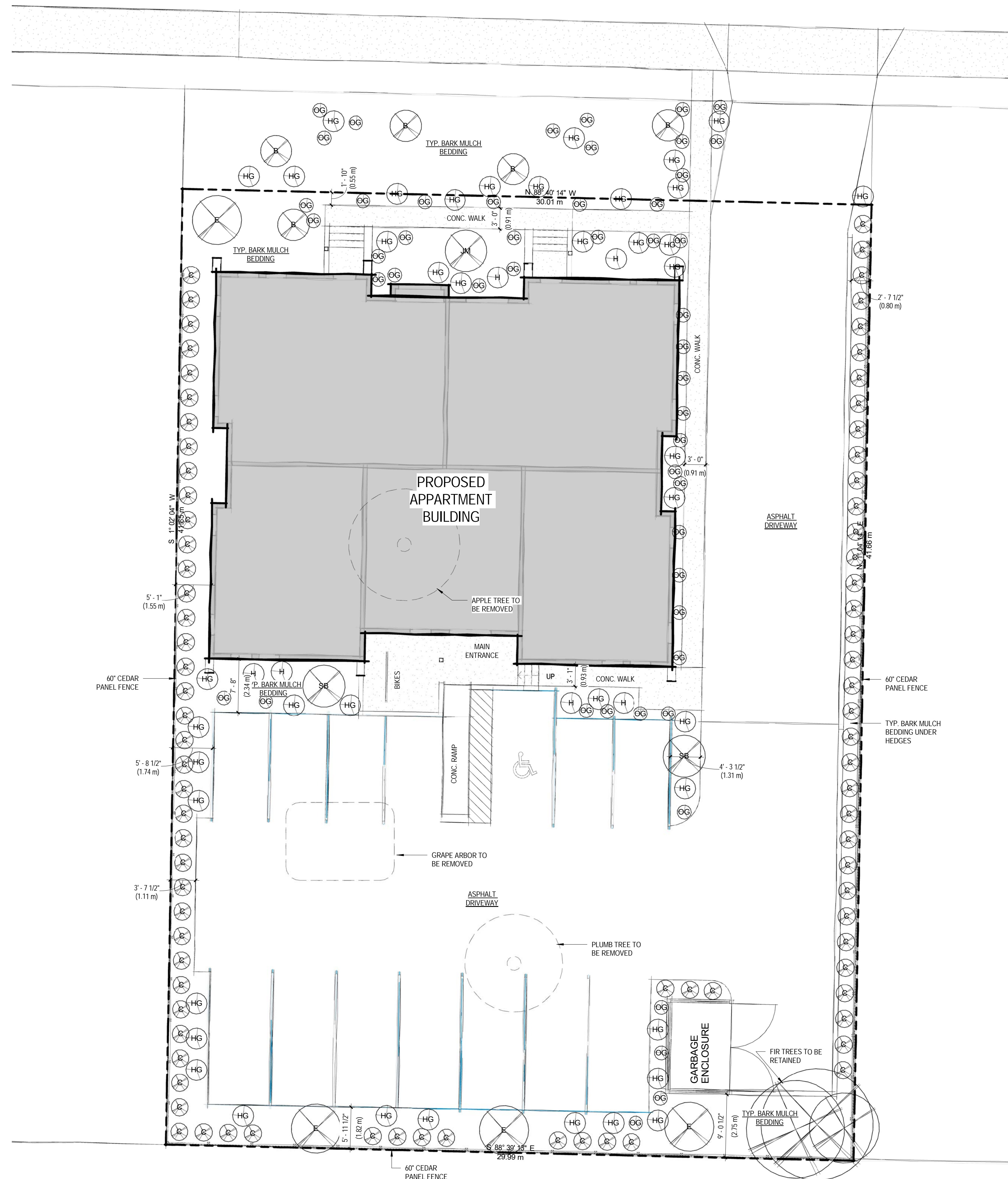
1 LANDSCAPE PLAN 1/8" = 1'-0"
